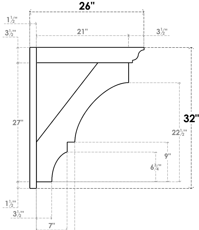
SIDE PROFILE
